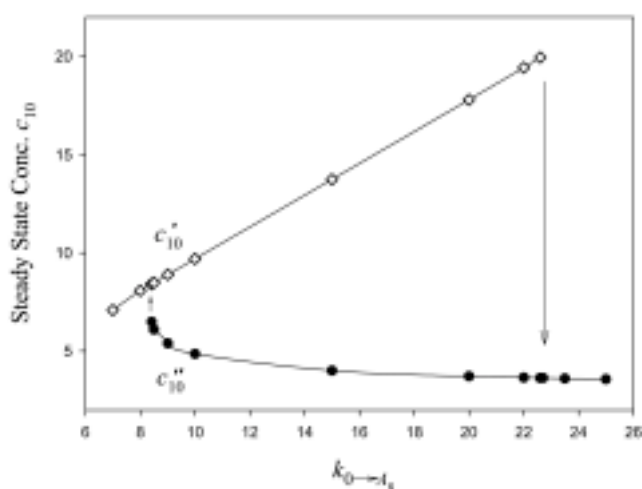
Fig. 2. The change of the steady state concentration c_{10} with the flow rate k_{0 \rightarrow A_8} for network (8).
